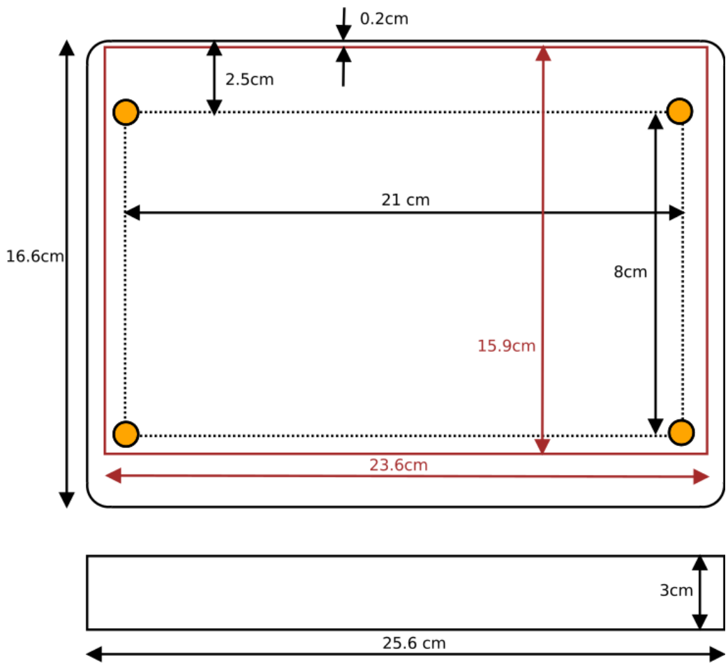
KUEHNCUT panel dimensions
