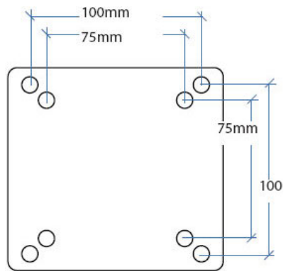
KUEHNCUT Touch PC VESA 100x100 dimensions
